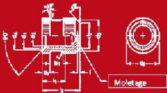
Form Q cylindrical with no spigot l1 H d1
