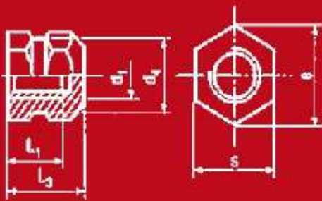
Forme P HEX with no spigot l1 H d1
