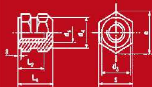
Forme R HEX with spigot l2 H 1,5 d1
